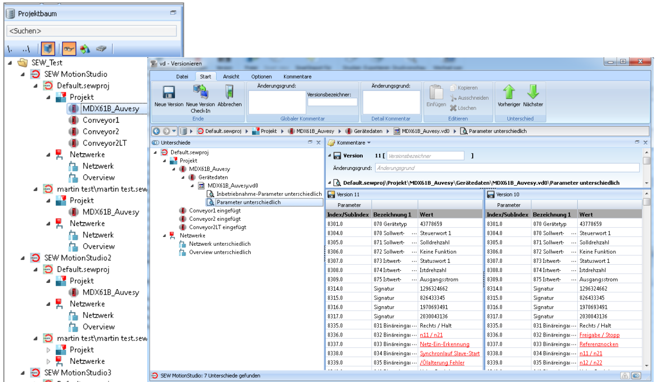
Fig. 1: Integrated SEW MOVITOOLS project tree
